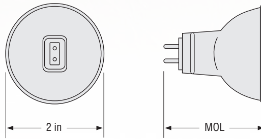
GU5.3 Base
