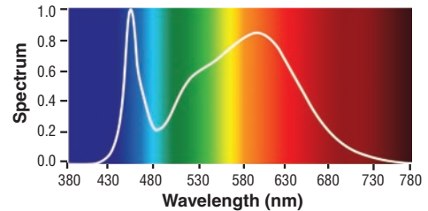
Item 3000678 25.5W LED T5 DR, NW40
