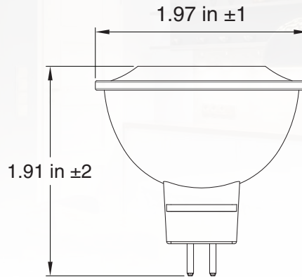
GU5.3 Base
